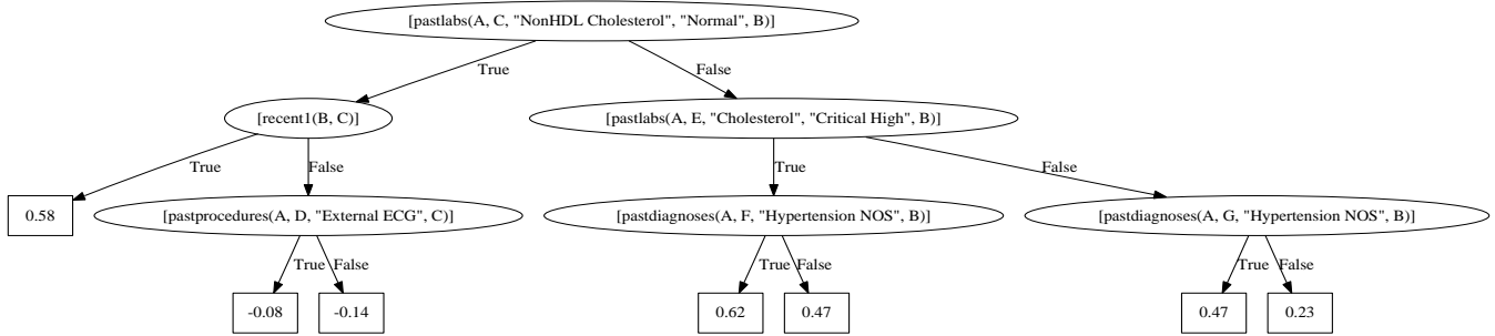
Figure 4: The first learned tree in the RFGB forest
